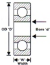
Ball Bearing with Poly Acetyl Outer, IMS Unground Inner & Carbon Balls
